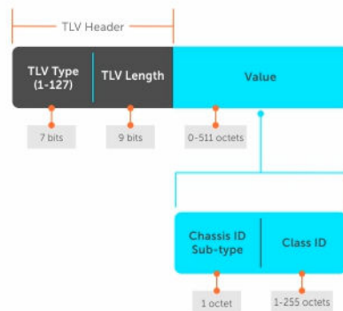
Figure 66. Type, Length, Value (TLV) Segment
